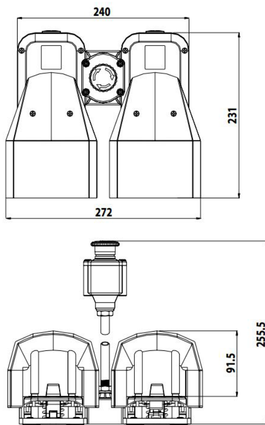
Double footswitch
