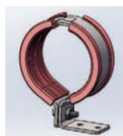
fixing clamp Ø70 mm, stainless steel A4, angle plug, wall clearance 70 mm
